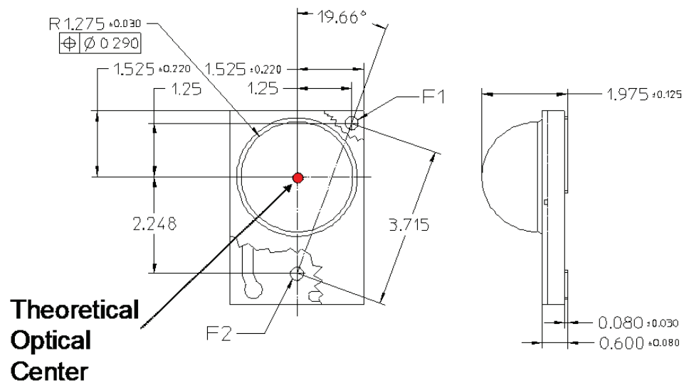
Figure 2. The most accurate method to find the theoretical optical center and the center of the dome is by using the fiducials located on the front side of the LUXEON Rebel LED. Dimensions in mm.
