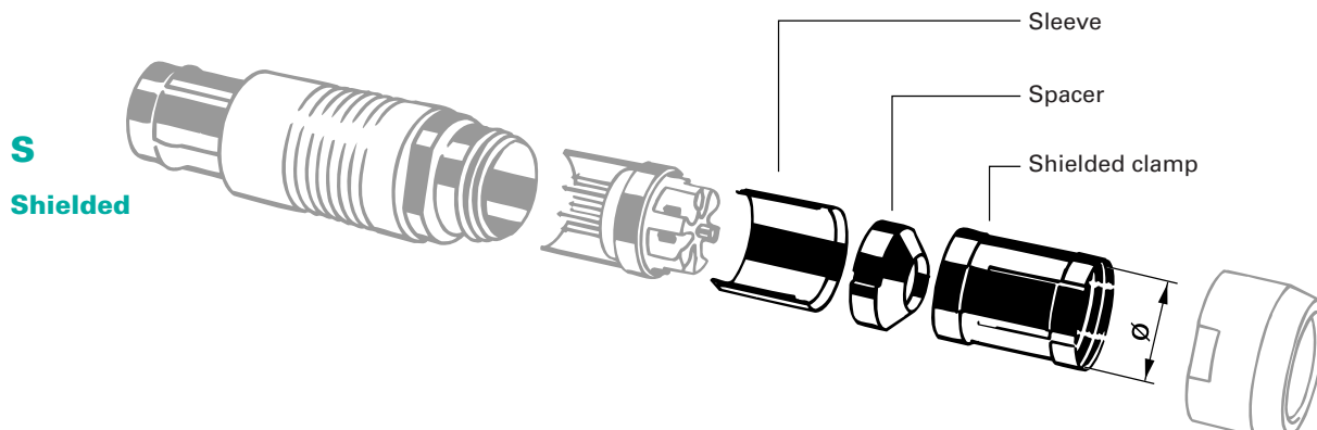
Shielded cable clamps and spacers for shielded or unshielded cables.
