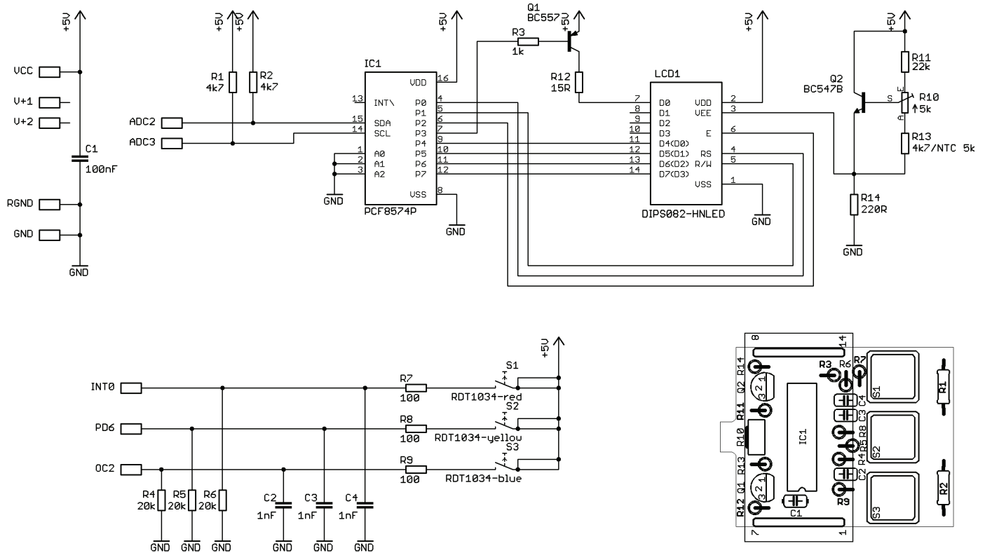
Circuit ARX-DSP
