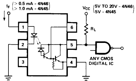
CMOS Interface
