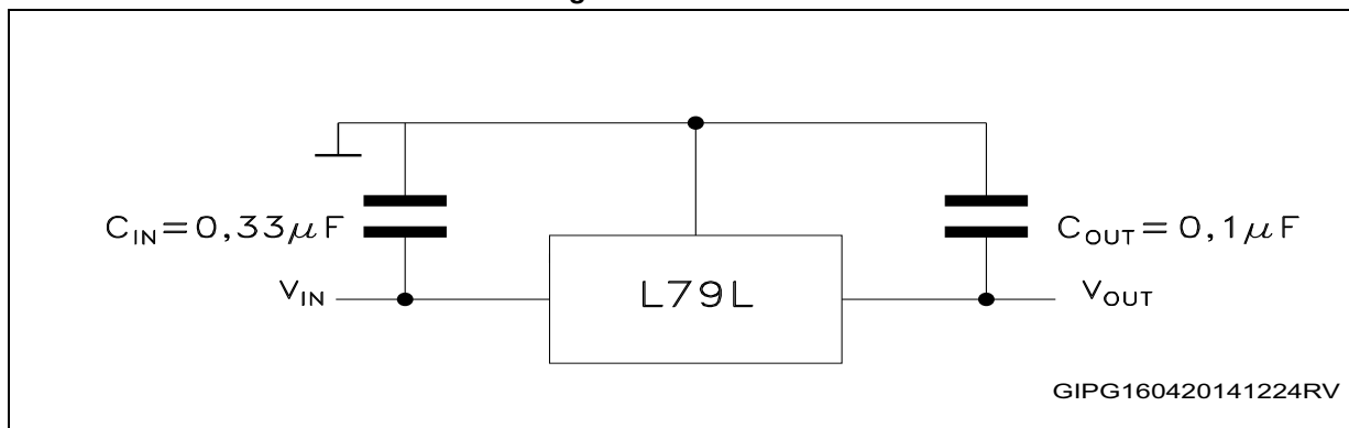
Figure 3. Test circuit
