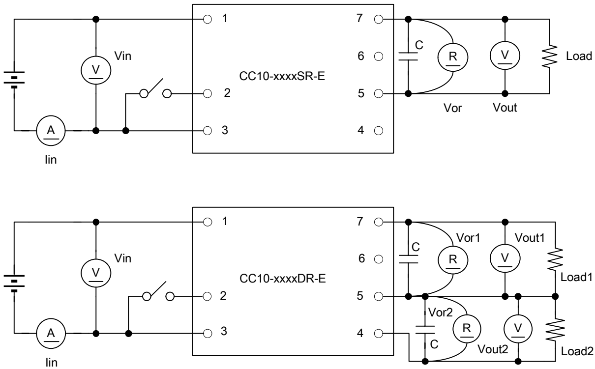
[5] Test Circuit
