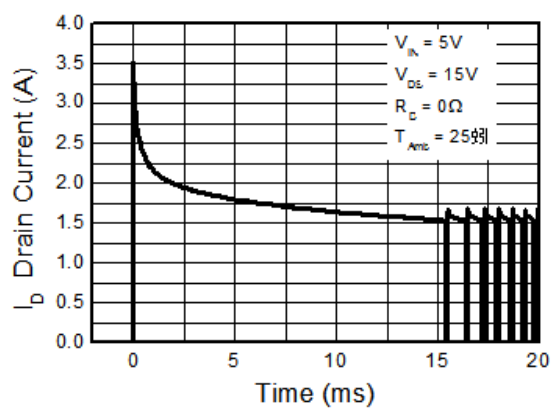
Typical Short Circuit Protection
