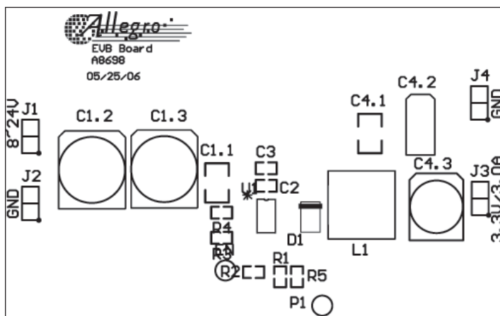
Silkscreen Layer
