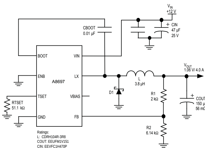
Circuit for 12 V step down to 1.06 V at 4 A
