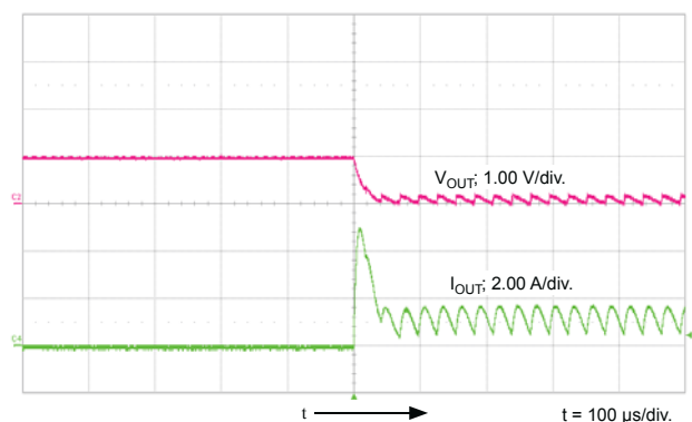
Short Circuit
