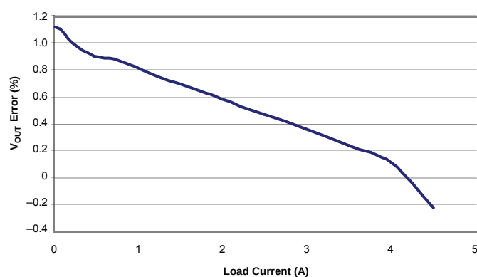
Load Regulation
