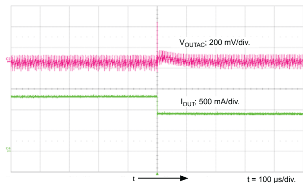
Load Transient, Step Down I_{OUT} = 1.6 \text{ to } 0.8 \text{ A}
