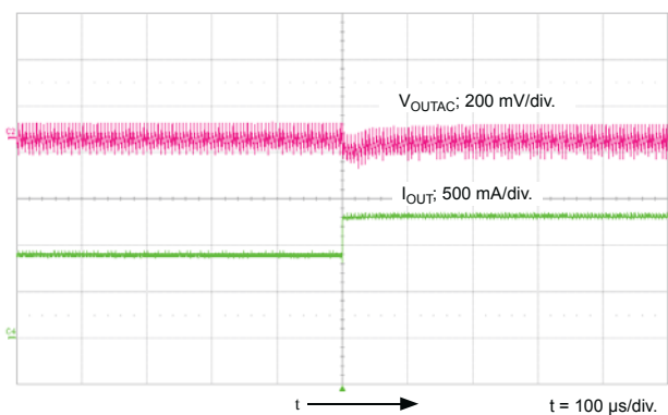
Load Transient, Step Up I_{OUT} = 0.8 \text{ to } 1.6 \text{ A}
