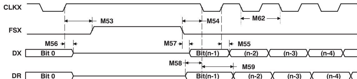
Figure 6-53. McBSP as SPI: CLKSTP = 11b, CLKXP = 1
