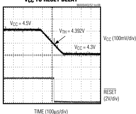
V_{CC} TO RESET DELAY
