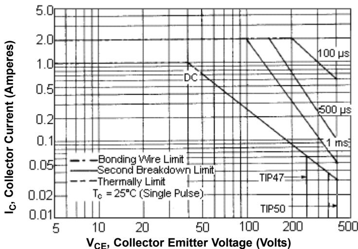
Figure - 6 Active Region Safe Operating Area
