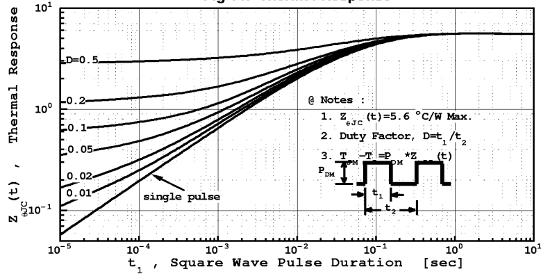
Fig 11. Thermal Response
