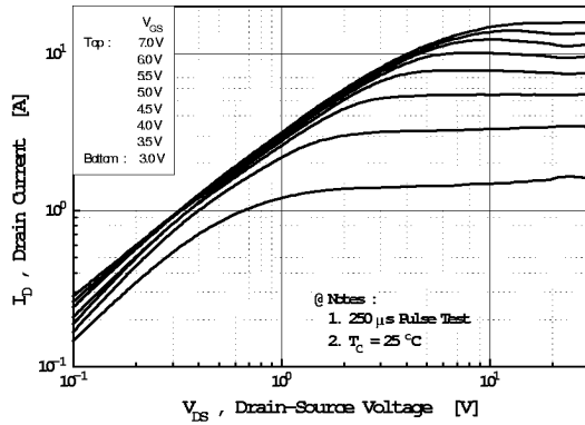
Fig 1. Output Characteristics
