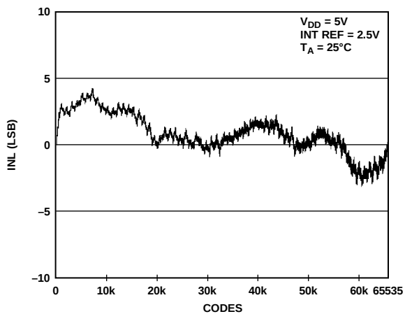
Figure 13. INL AD5668-2/AD5668-3
