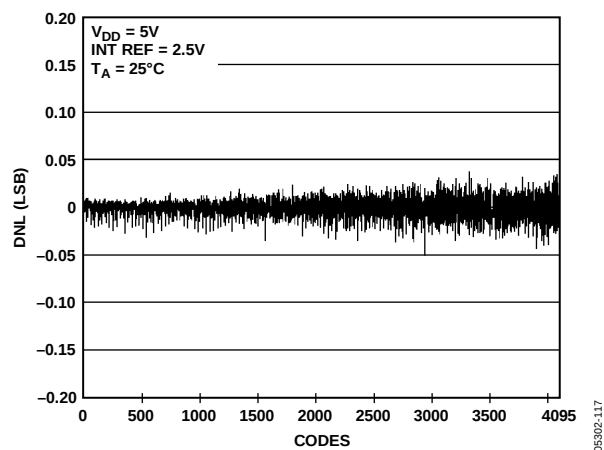
Figure 18. DNL AD5628-2
