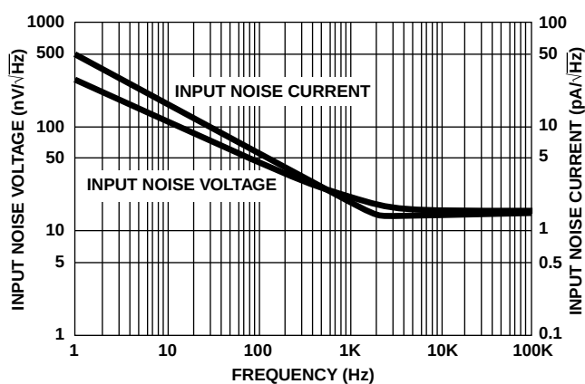
FIGURE 17. INPUT NOISE CHARACTERISTICS
