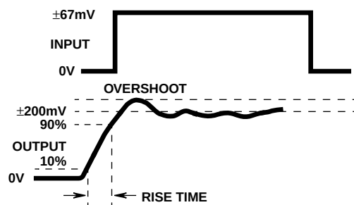
FIGURE 2. TRANSIENT RESPONSE
