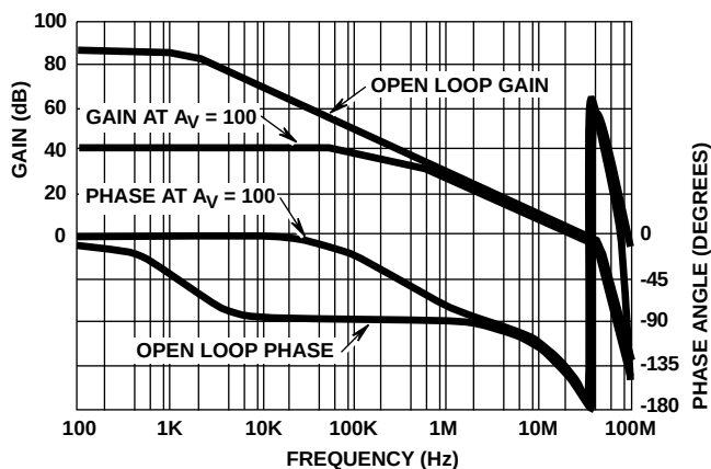
FIGURE 15. FREQUENCY RESPONSE
