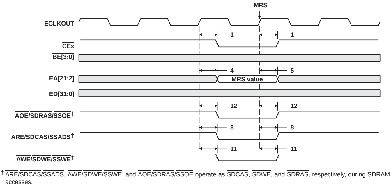
Figure 43. SDRAM MRS Command
