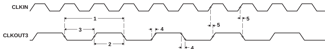
Figure 30. CLKOUT3 Timings
