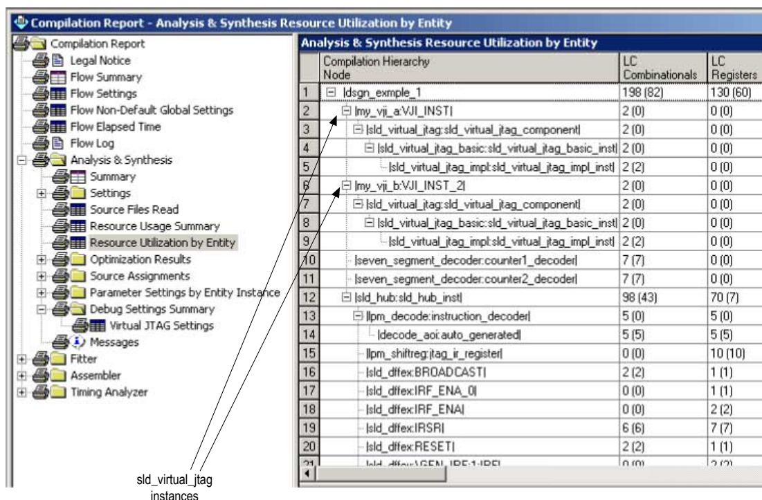
Figure 15: Logic Resources Utilized
