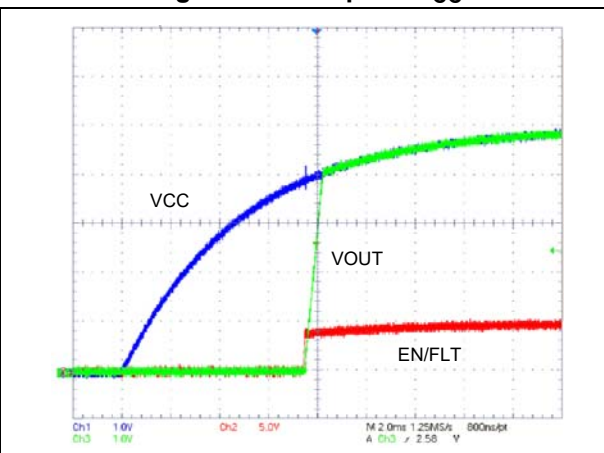
Figure 10. Startup @ heavy load
