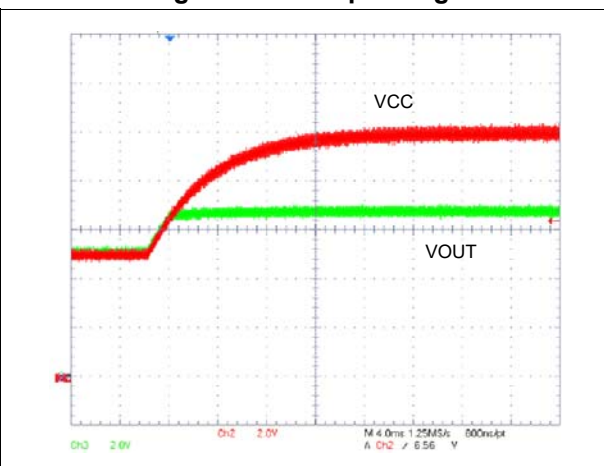
Figure 12. Clamp voltage
