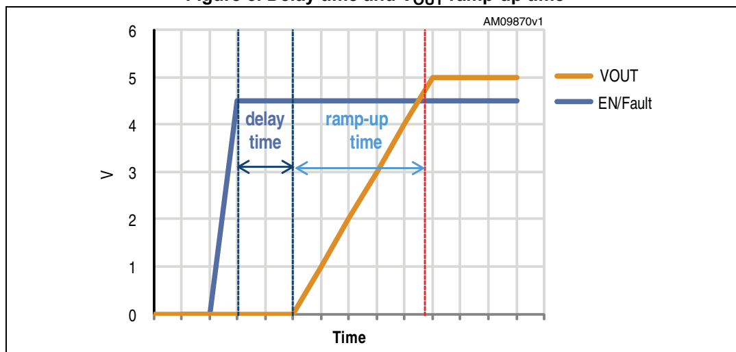
Figure 5. Delay time and V_{OUT} ramp-up time
