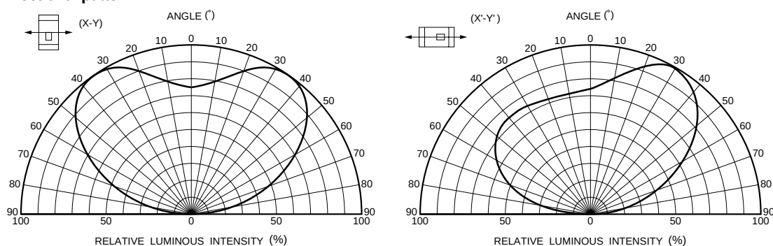
Fig. 1 Directional pattern
