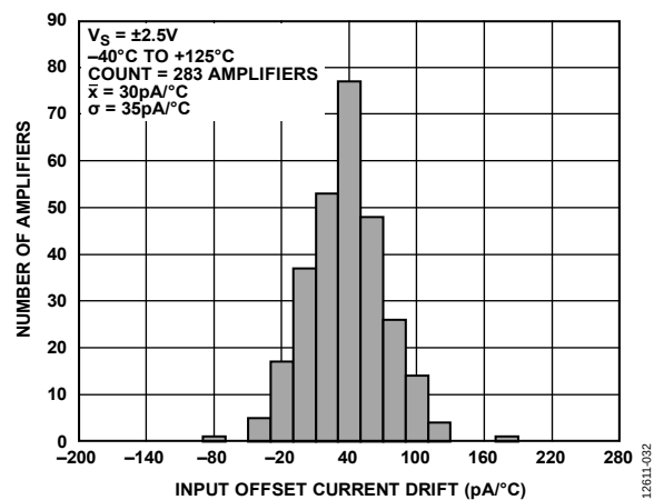
Figure 32. Input Offset Current Drift Distribution, V_{CM} = 0\text{V}
