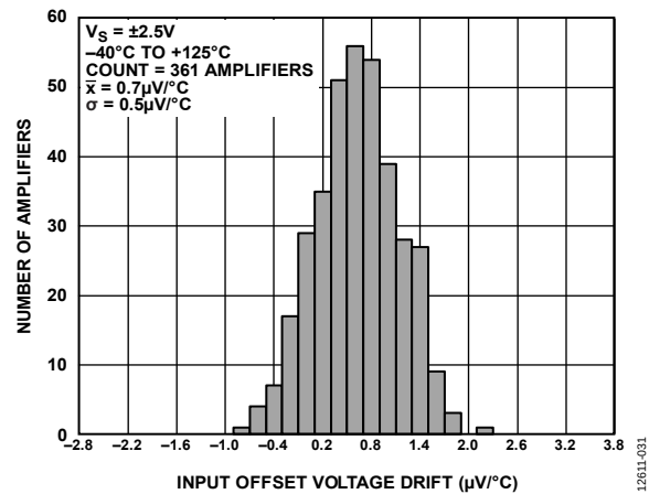
Figure 31. Input Referred Offset Voltage Drift Distribution, V_{CM} = 0\text{V}
