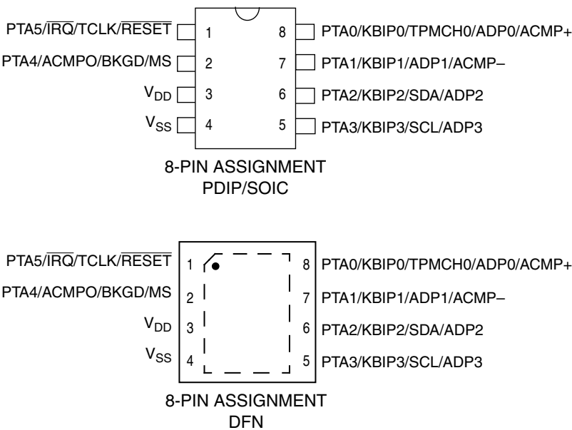
Figure 2-1. 8-Pin Packages
