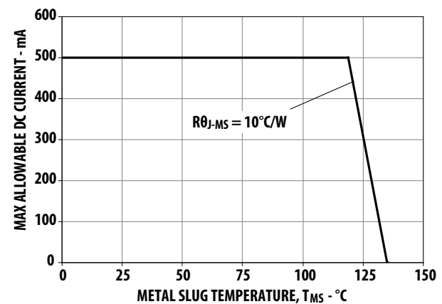
Figure 23. Maximum Forward Current vs. Metal Slug Temperature. Derated based on T_{JMAX} = 135^\circ\text{C} , R\theta_{MS} = 10^\circ\text{C/W} .
