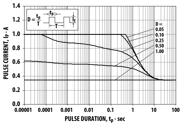
Figure 18. Maximum pulse current vs. pulse duration. Derated based on T_A = 25^\circ\text{C} , R\theta_{JA} = 50^\circ\text{C/W} .
