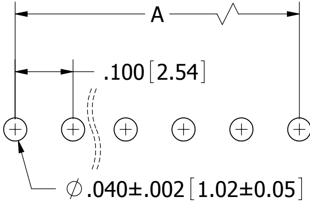
RECOMMENDED PCB LAYOUT SINGLE ROW
