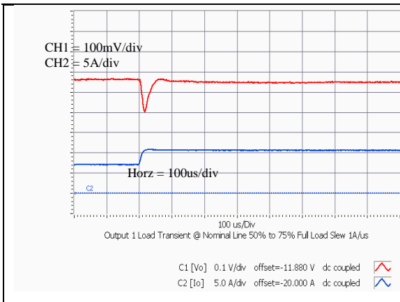
Vo=12V Typical output voltage transient response to load step from 50% to 75% of full load with output current slew rate of 1A/uS. (Cext = 3x47uF ceramic capacitor)
