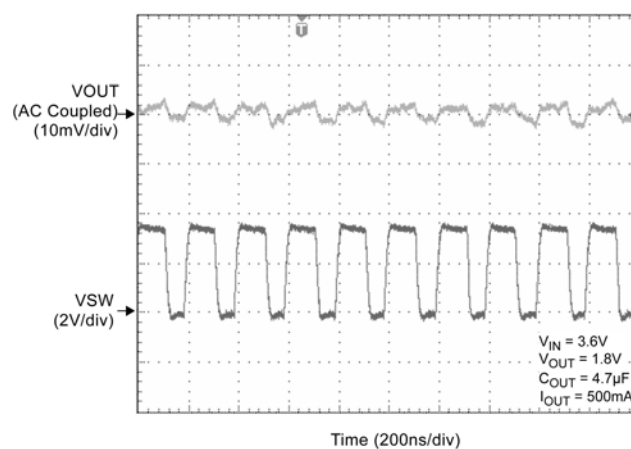
Switching Waveform
