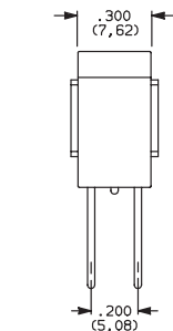
T201J1AVBE2 Vertical Actuation DPDT
