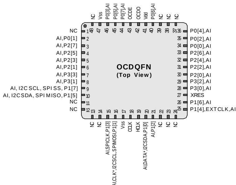
CY8C20000 OCD PSoC Device
