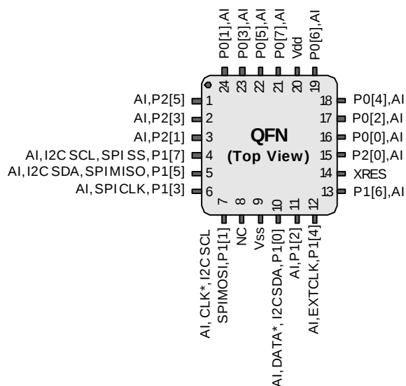
CY8C20334 24-Pin PSoC Device
