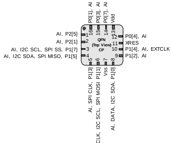
CY8C20234 16-Pin PSoC Device
