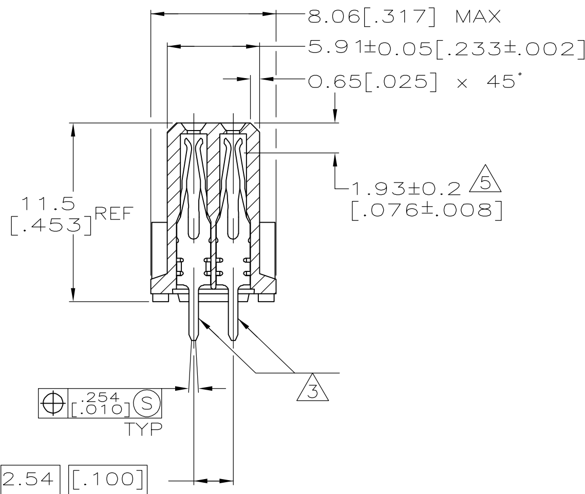
SECTION X-X
