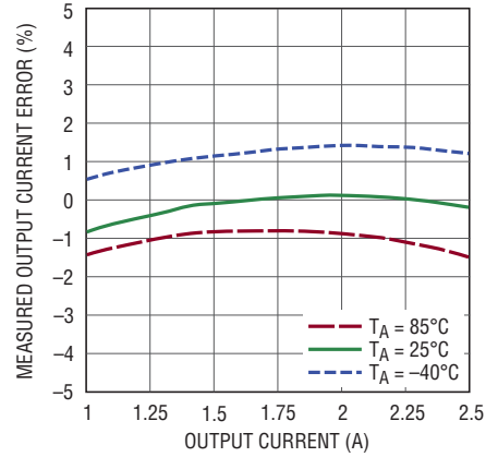
Output Current Monitor Error vs Output Current
