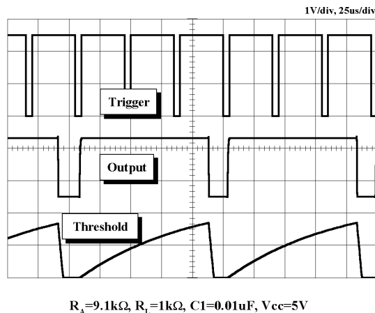
Figure 8. Waveforms of Frequency Divider Operation
