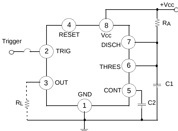
Figure 1. Monoatable Circuit
