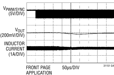
Phase-Locked Loop Acquisition, V_{IN} = 24\text{V} 1.2MHz Clock
