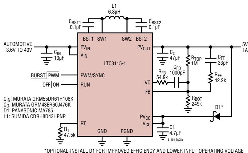
750kHz Automotive 5V Regulator with Cold Crank Capability
