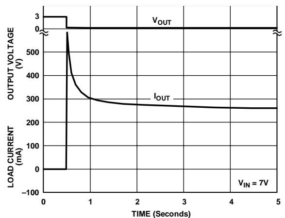
Figure 17. Short-Circuit Current
