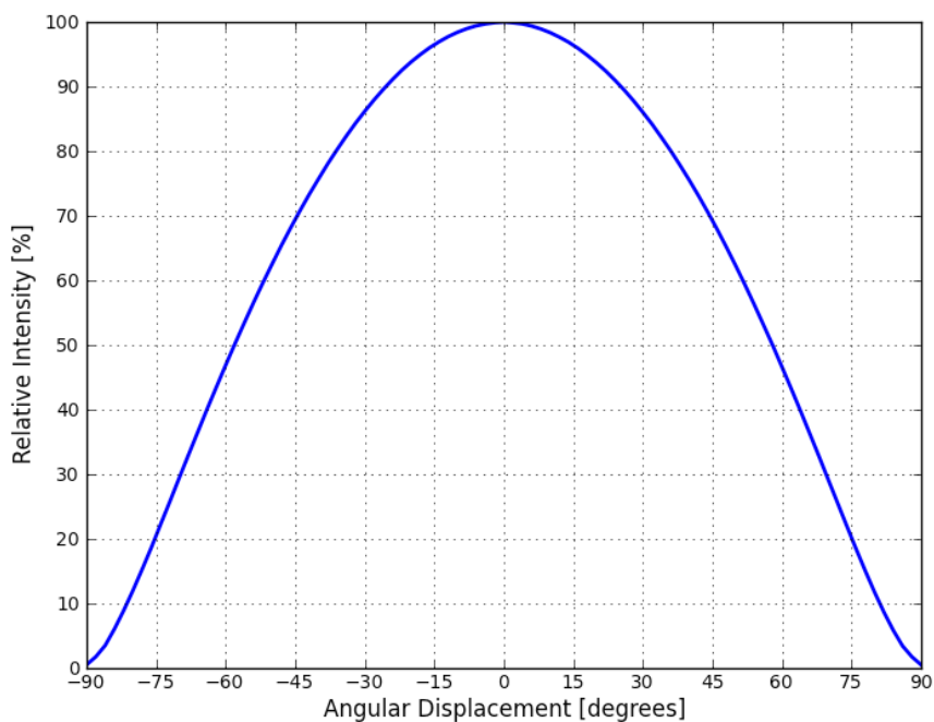
Figure 9. Typical spatial radiation pattern, L135-xx80-0xHV-00001.
