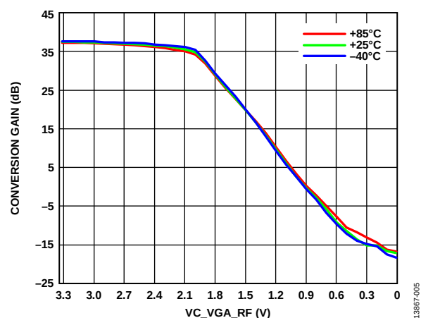
Figure 5. Conversion Gain vs. VC\_VGA\_RF at RF = 1 GHz, 56 MHz Filter (RF Input Power = -40 dBm, VC\_VGA\_IF = 0 V)
