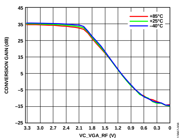
Figure 8. Conversion Gain vs. VC\_VGA\_RF at RF = 2 GHz, 56 MHz Filter (RF Input Power = -40 dBm, VC\_VGA\_IF = 0 V)
