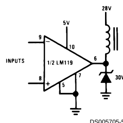
Relay Driver
