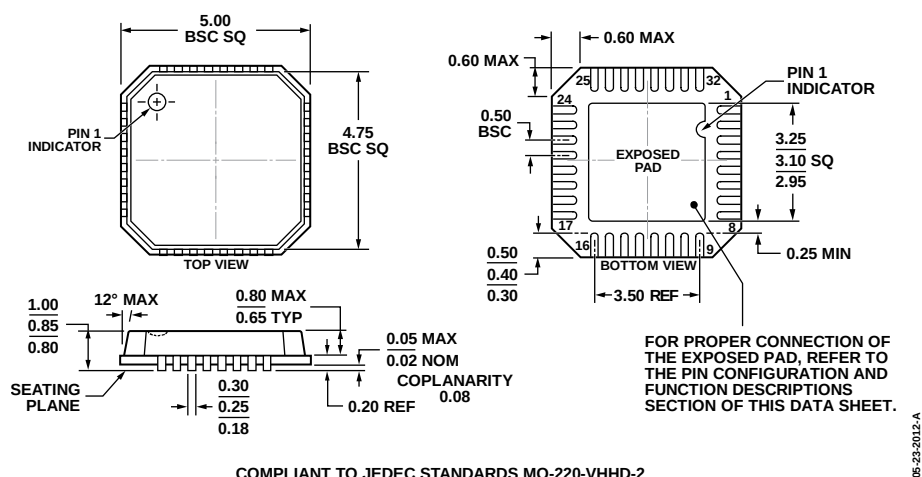
Figure 36. 32-Lead Lead Frame Chip Scale Package [LFCSP_VQ] 5 mm × 5 mm Body, Very Thin Quad (CP-32-2) Dimensions shown in millimeters
