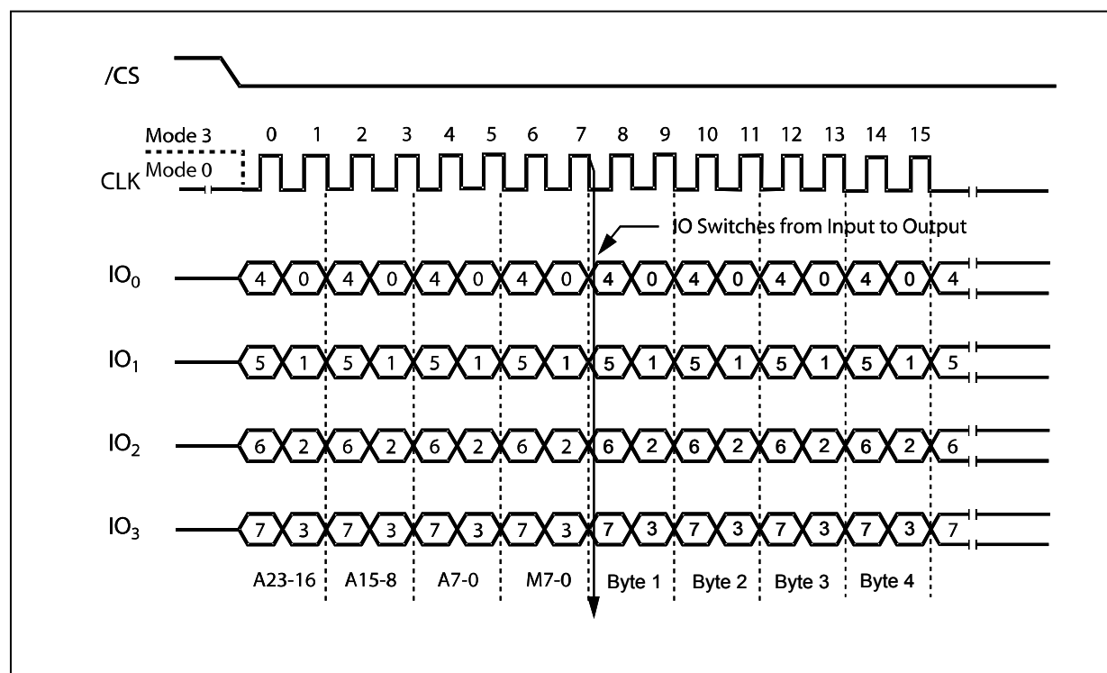
Figure 15b. Octal Word Read Quad I/O Instruction Sequence Diagram (M7-0 = Axx)
