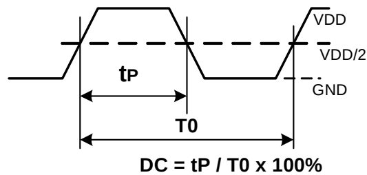
Figure 3. Output Duty Cycle (DC)
