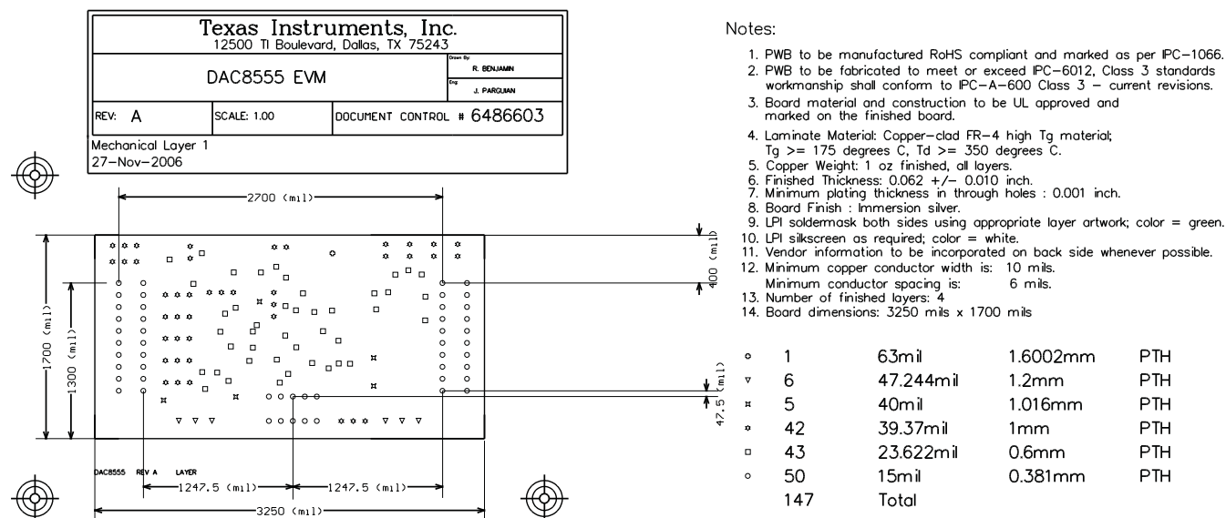
Figure 8. DAC8555EVM—Drill Drawing
