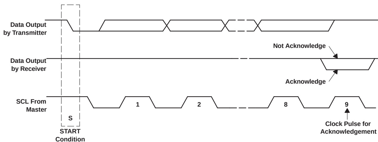
Figure 47. Acknowledge on the I 2 C Bus
