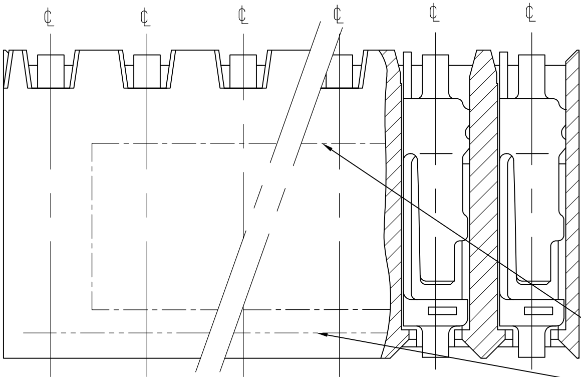
SECTION B-B/TOPVIEW
