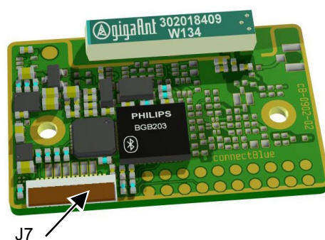
Picture 6: Flexfilm connector, J7.
