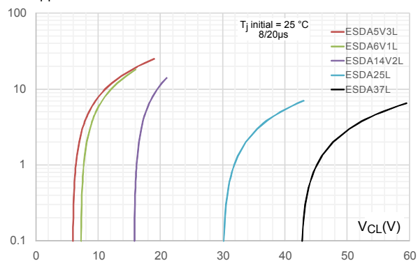
Figure 5: Variation of clamping voltage versus peak pulse current (max. values, 8/20 \mu s waveform)
