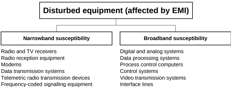
Fig. 6 Disturbed equipment
