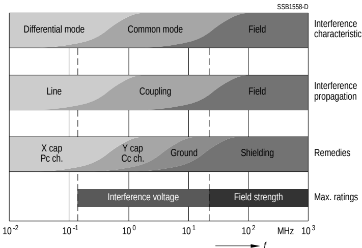
Fig. 2 Frequency range overview
