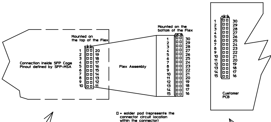
Industrial SFP Circuit Wiring Scheme
