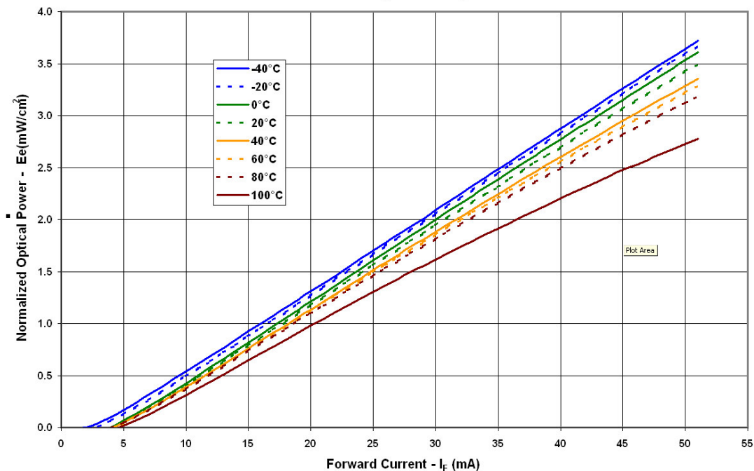
Optical Power - E_e(\text{mW/cm}^2) vs Forward Current - I_F vs Temperature - T_A
