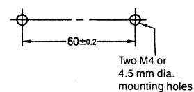
Mounting holes
