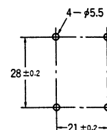
Front mounting
