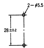
Mounting holes Side mounting
