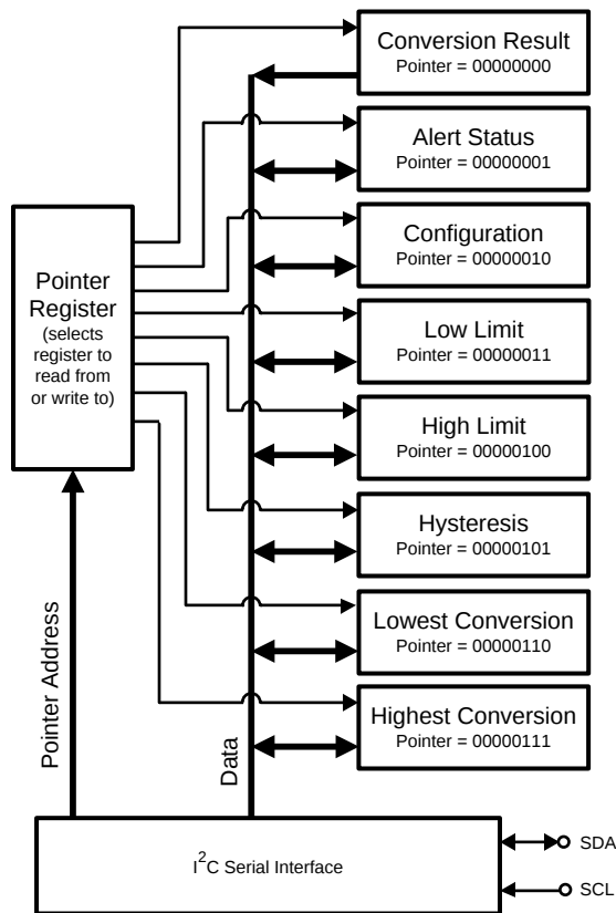
Figure 21. Register Structure
