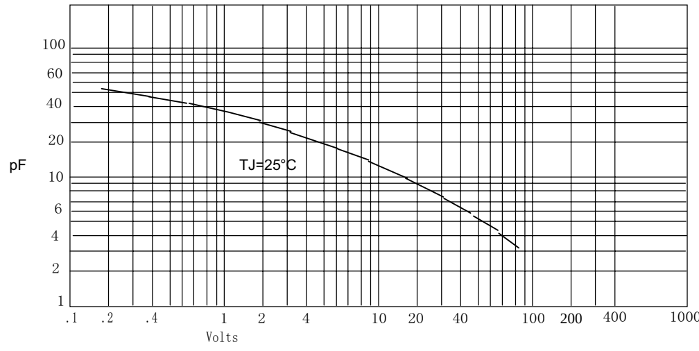
Figure 4 Junction Capacitance
