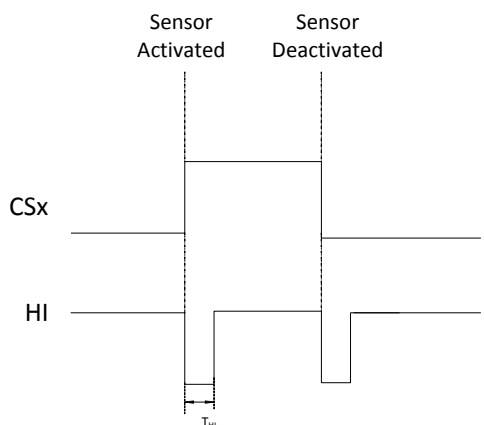
Figure 11. Host Interrupt Line with CSx Buttons Touched Separately
