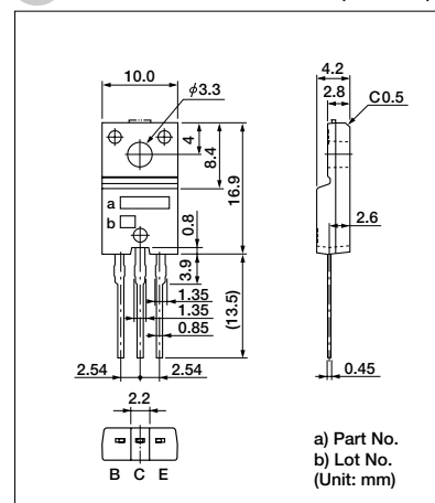
External Dimensions TO220F (full-mold)
